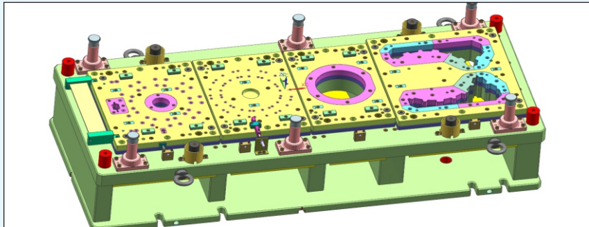
Bottom Half Assembly for Driven Plate Progressive Tool
