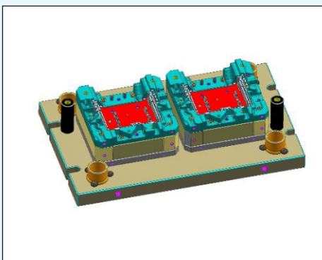
Trim Tool Top Half for ECU Cover
