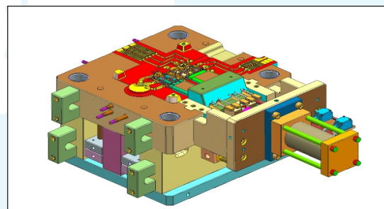
Moving Half for Valve Body HPDC Die
