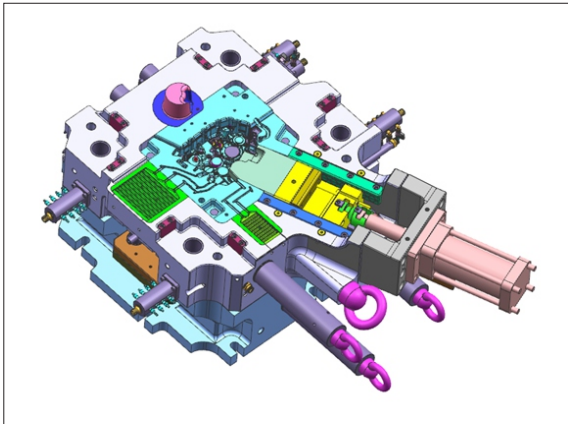
Crank Case RH Bottom Half Assembly
