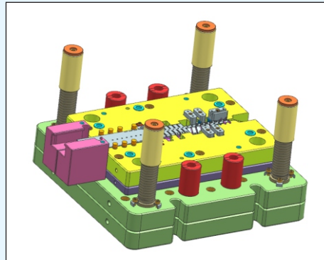
Progressive Tool for Terminal Box
