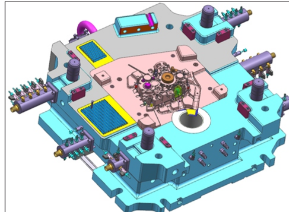
Crank Case RH Top Half Assembly
