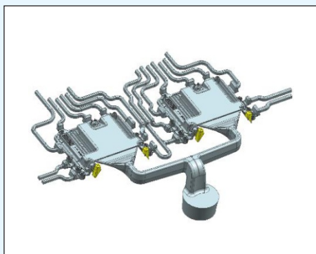
Shot Model for ECU Cover
