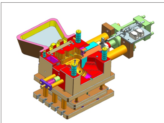
GDC Die for Thermostat Housing - Bottom Half
