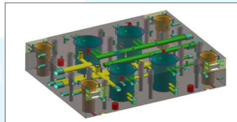
Cavity Plate
