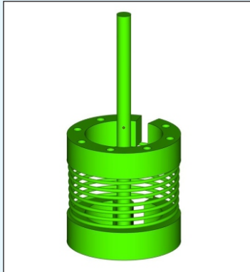
SOLENOID COIL
