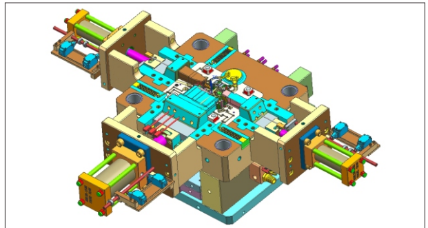
Solenoid Body - Moving Half
