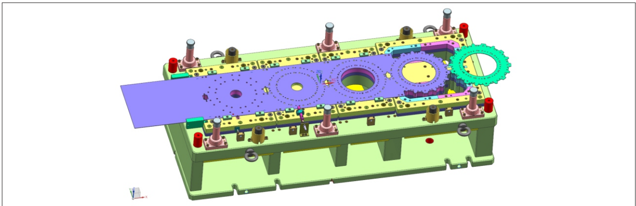
Progressive Tool For 430 Driven Plate
