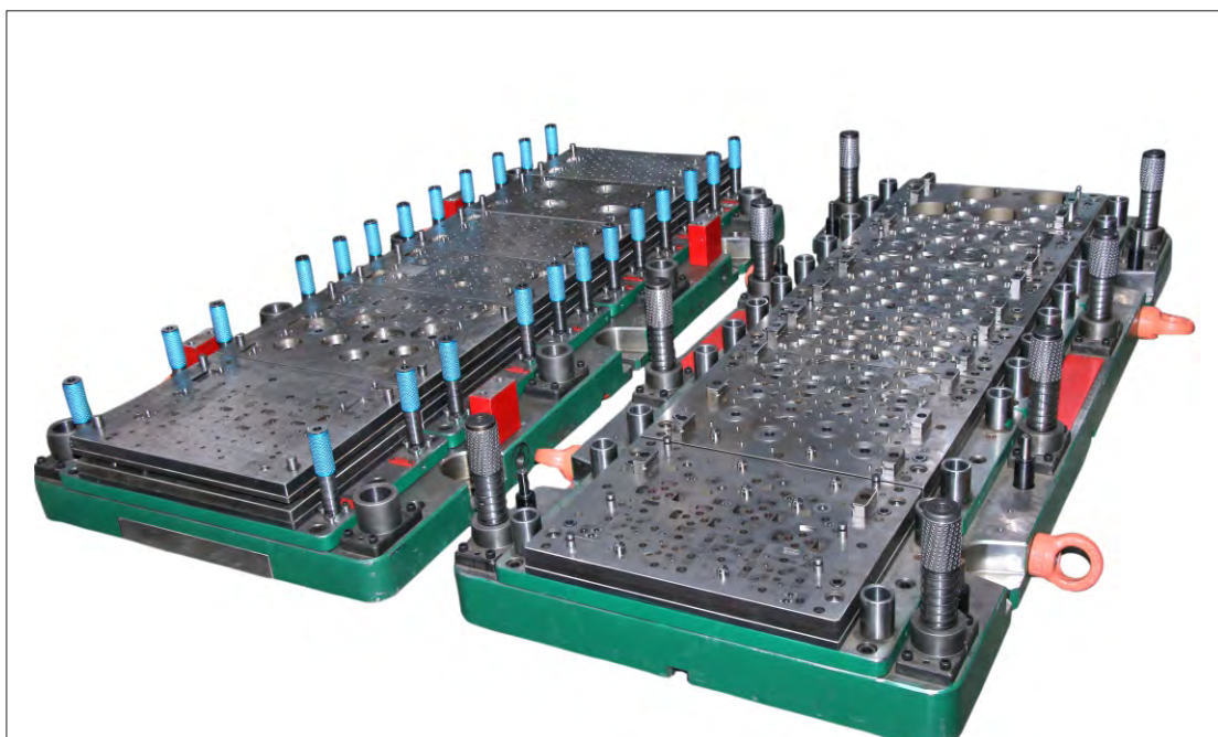
Four Row Progressive Tool for Retainer Plate developed by IGTR-Aurangabad
