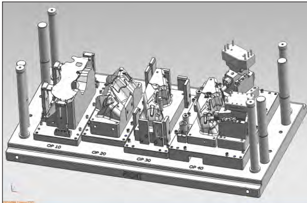
Designed & Manufactured Press Tool for Heat Shield & Component
